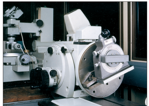
TB100 checking dividing head
