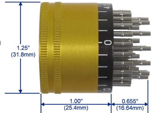
48DF-1/2 (Female)
